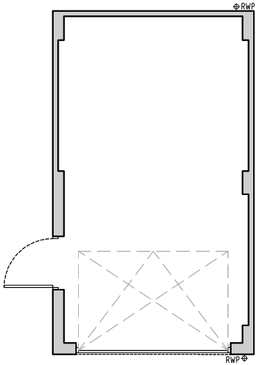
Ground Plan 1:100
