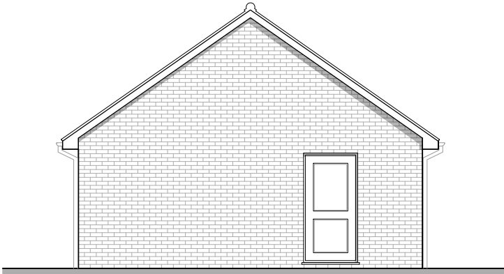
Left Flank Elevation 1:100
