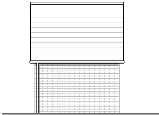
Rear Elevation 1:100
