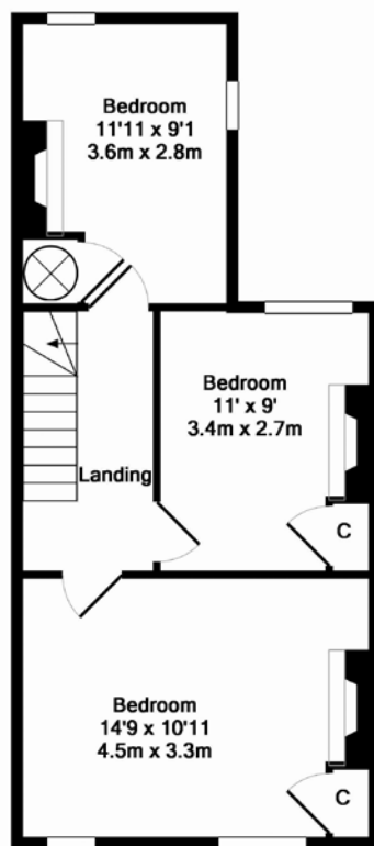
1st Floor Approx. Floor Area 432 Sq.Ft. (40.1 Sq.M.)
