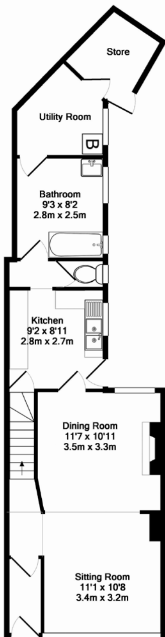
Ground Floor Approx. Floor Area 585 Sq.Ft. (54.3 Sq.M.)
