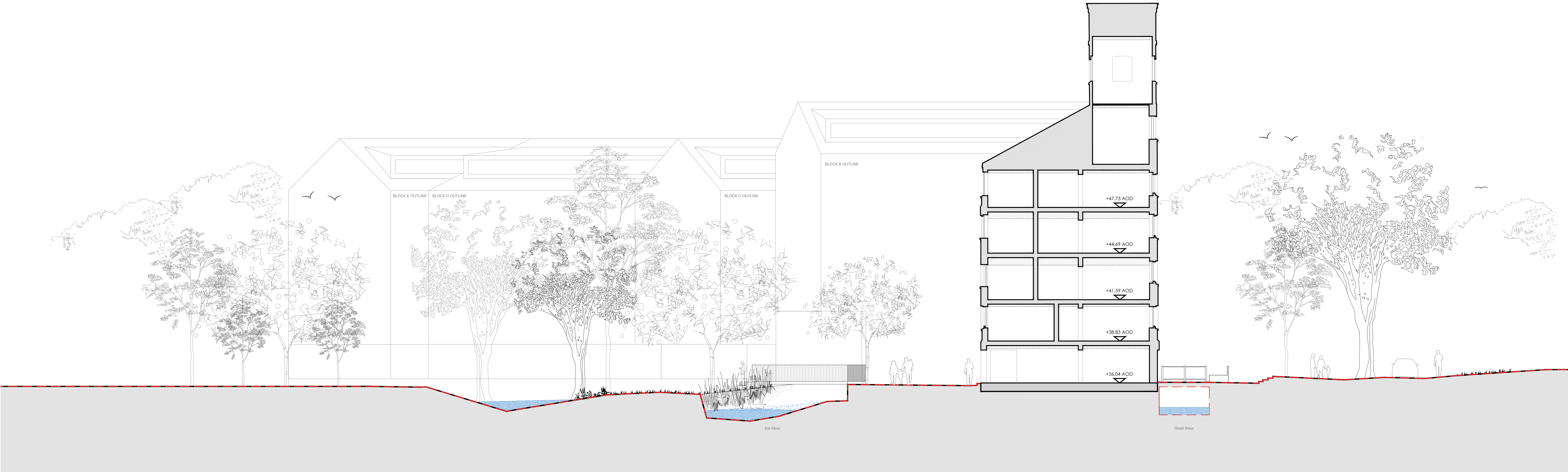
Proposed Section B-B Scale 1:100
