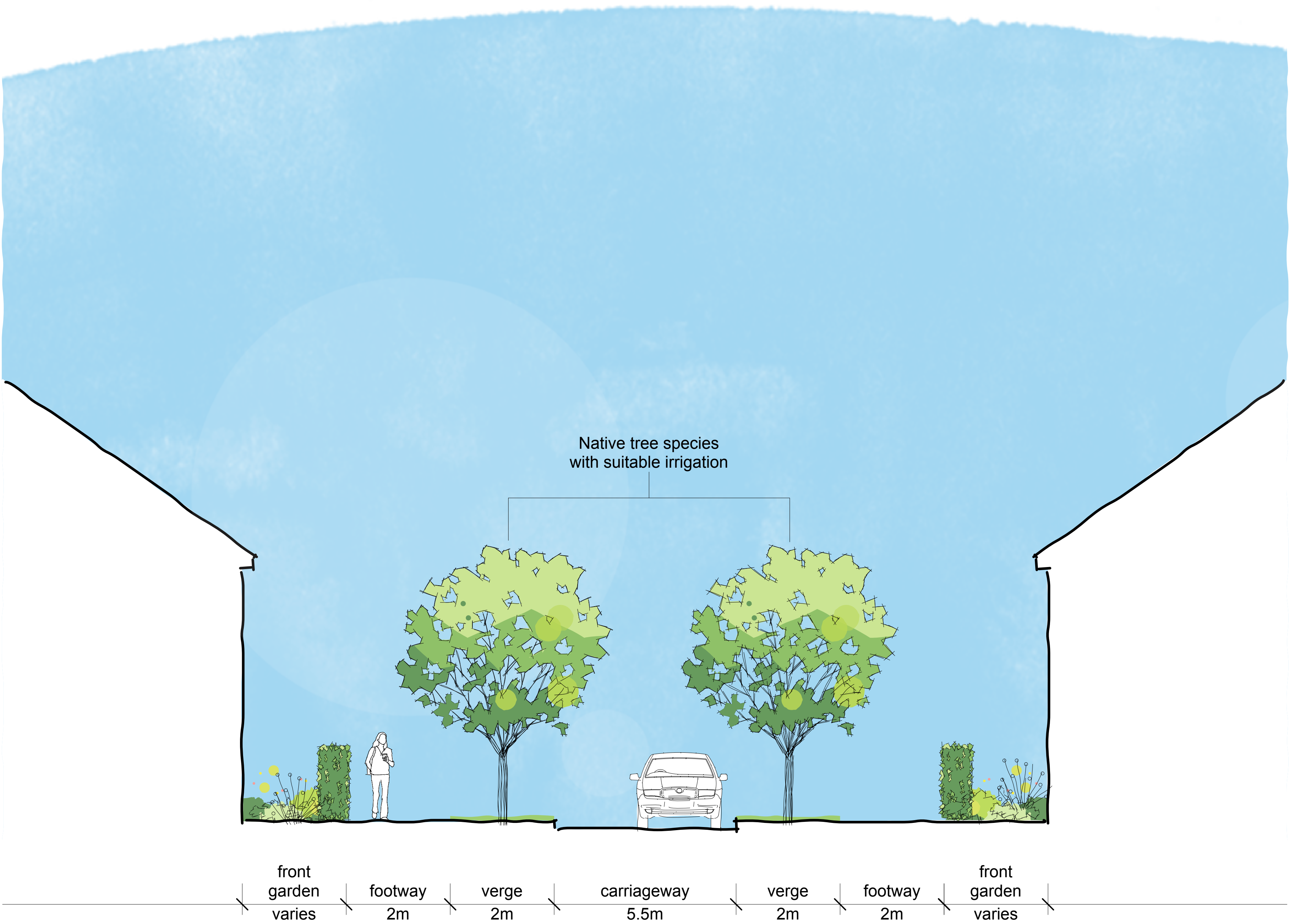
Section A - A Main Street
