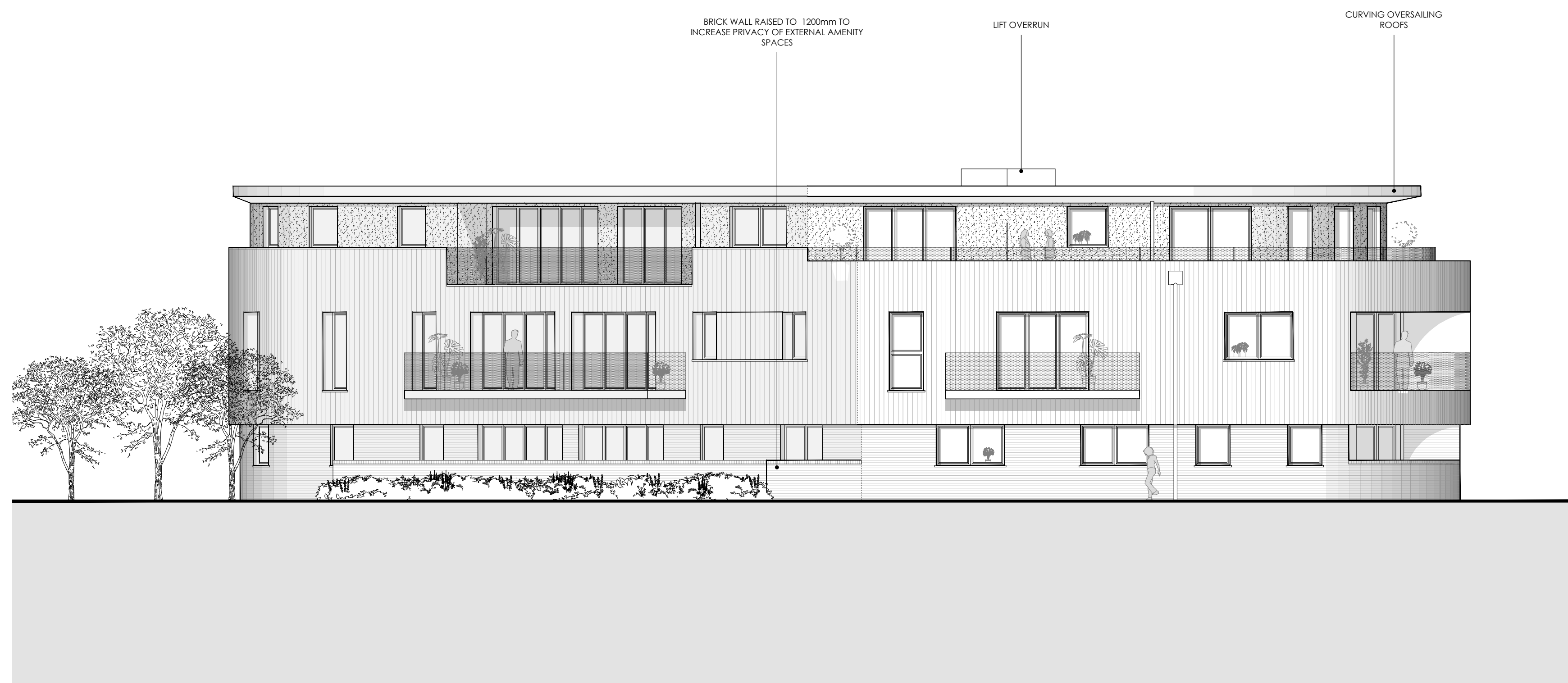
PROPOSED ELEVATION A-A SCALE 1:100 @ A1
