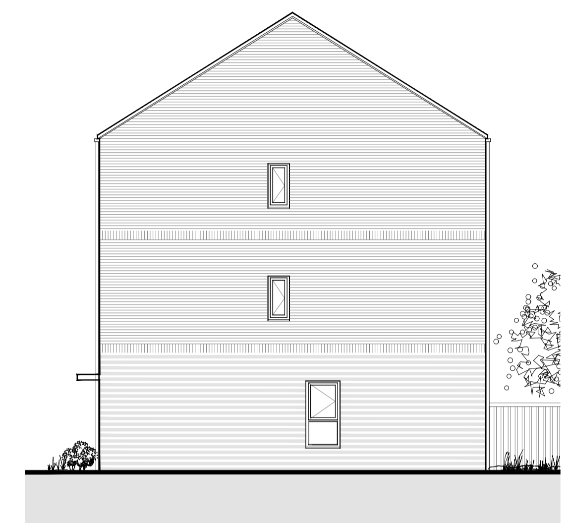
PROPOSED LEFT SIDE ELEVATION SCALE 1:100
