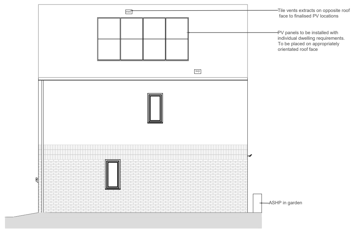
3 Bed Right Gable Elevation 1:100
