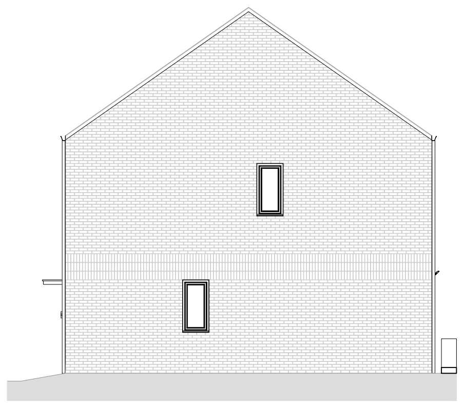
3 Bed Right Gable Elevation 1:100
