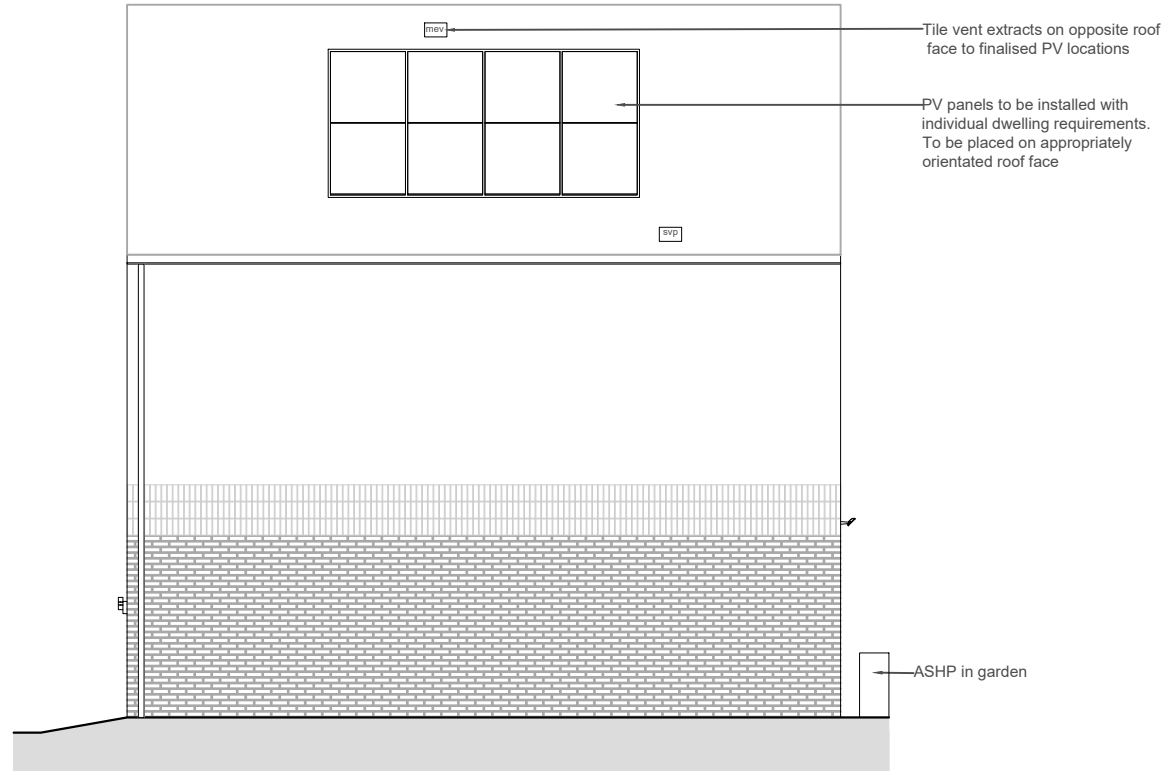
Right Gable Elevation 1:100
