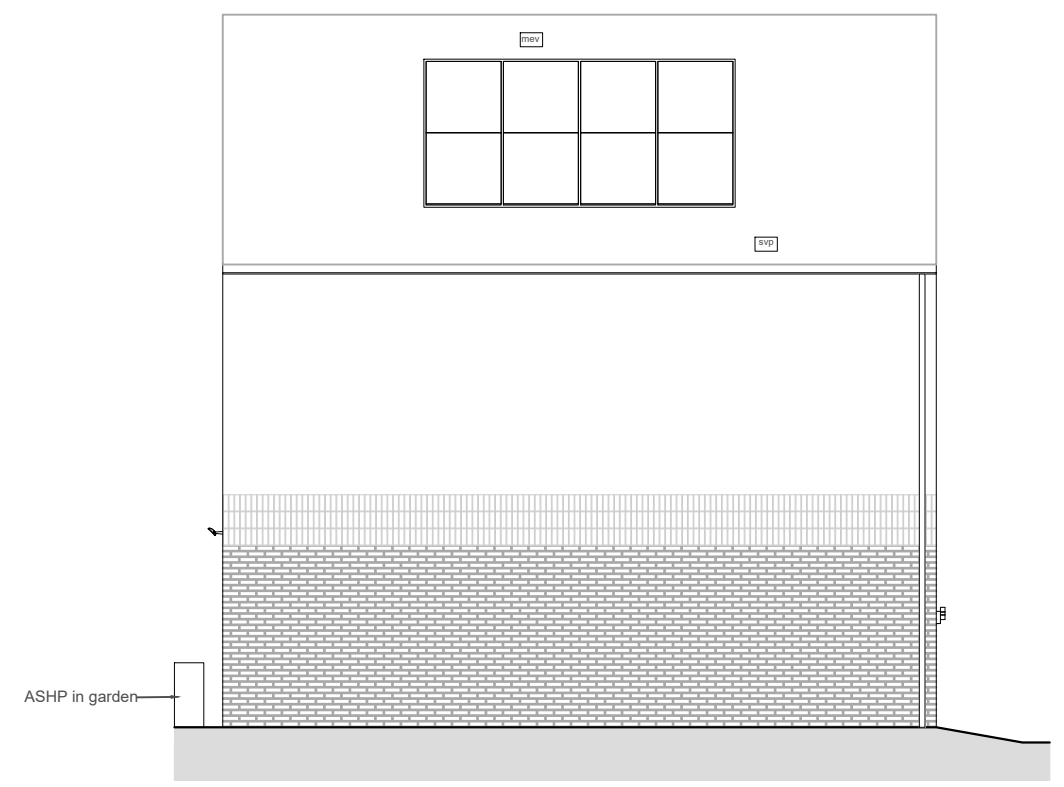
2 Bed Left Gable Elevation 1:100
