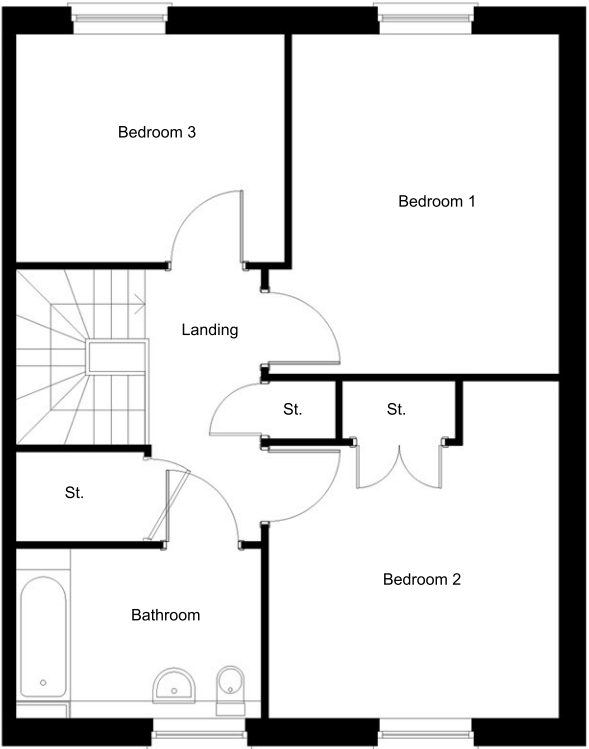
First Floor Plan - End (Right)
