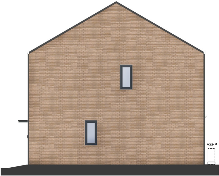
Gable Elevation (Right) Side window applies to Plots 1, 28, 43 + 71
