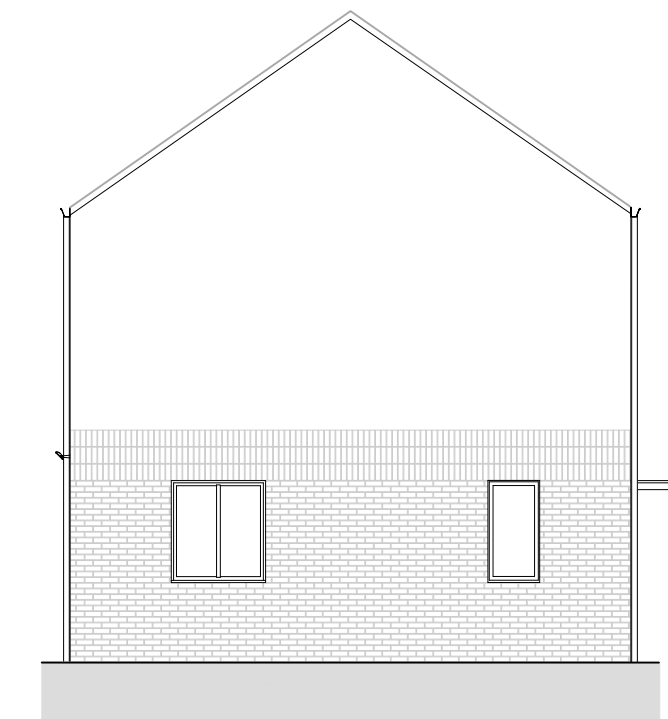
4 Bed Self-Build Left Gable Elevation * Windows applicable to Plots 35 & 45 only 1:100
