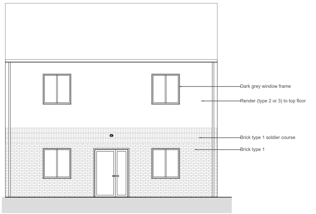
4 Bed Self-Build Rear Elevation 1:100
