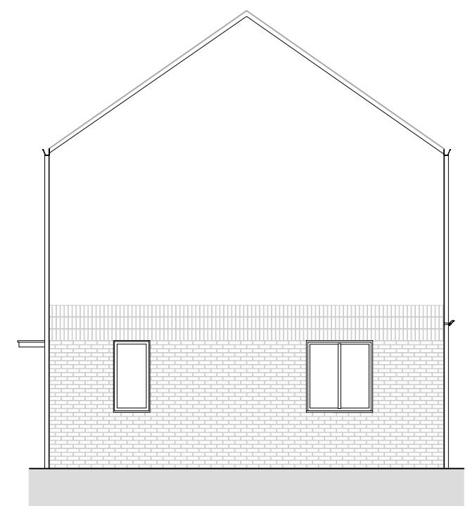
4 Bed Self-Build Right Gable Elevation * Windows applicable to Plots 35 & 45 only 1:100
