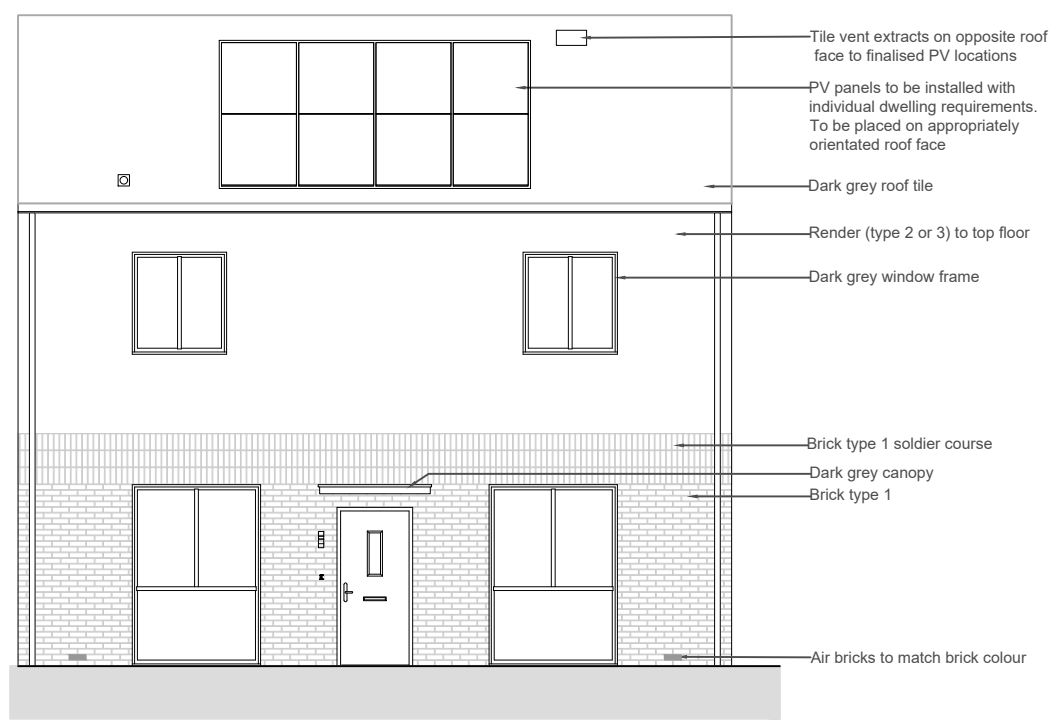
4 Bed Self-Build Front Elevation 1:100
