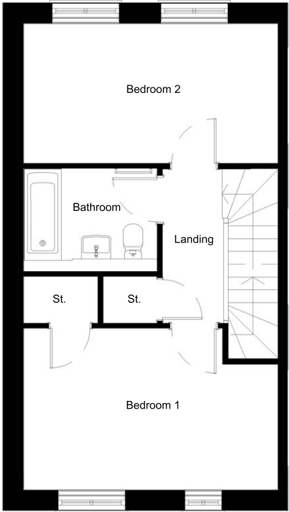
First Floor Plan - End (Left)
