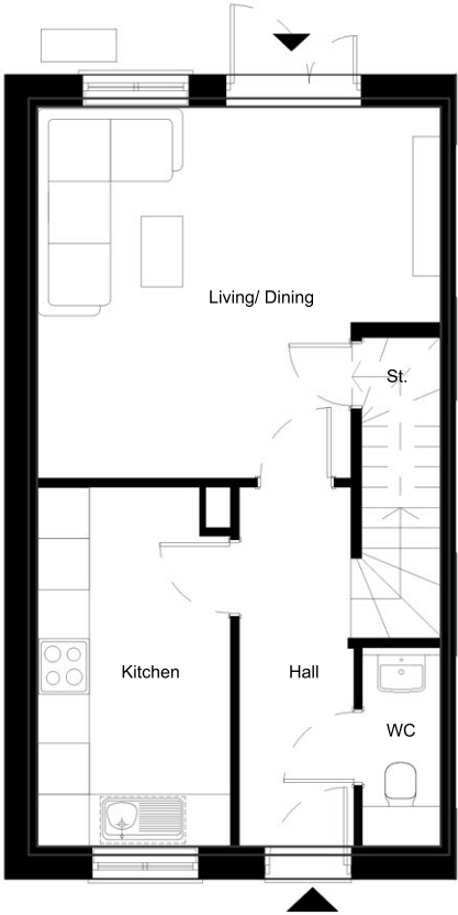
Ground Floor Plan - End (Left)
