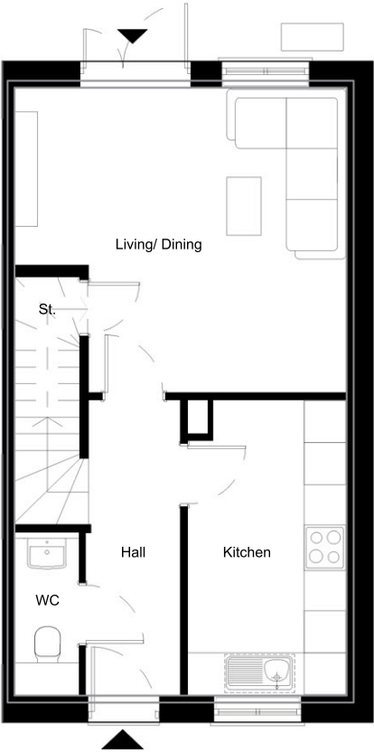
Ground Floor Plan - End (Right)
