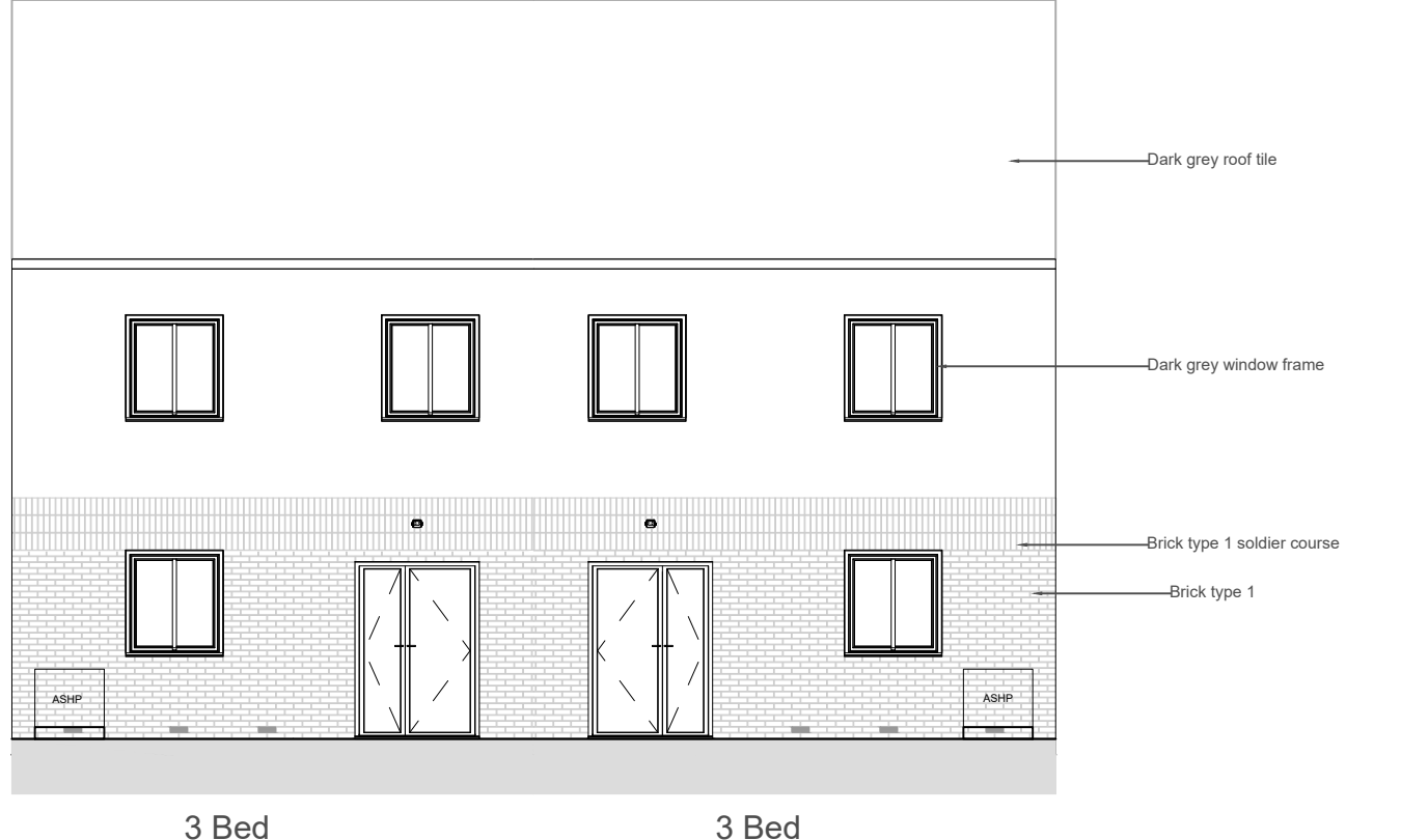
Rear Elevation 1:100
