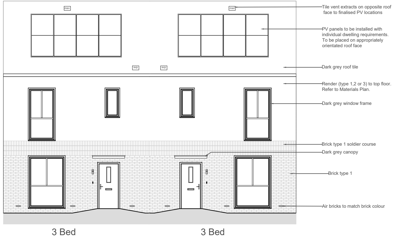
Front Elevation 1:100
