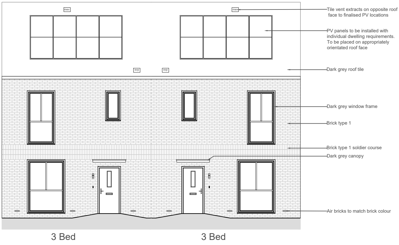
Front Elevation 1:100
