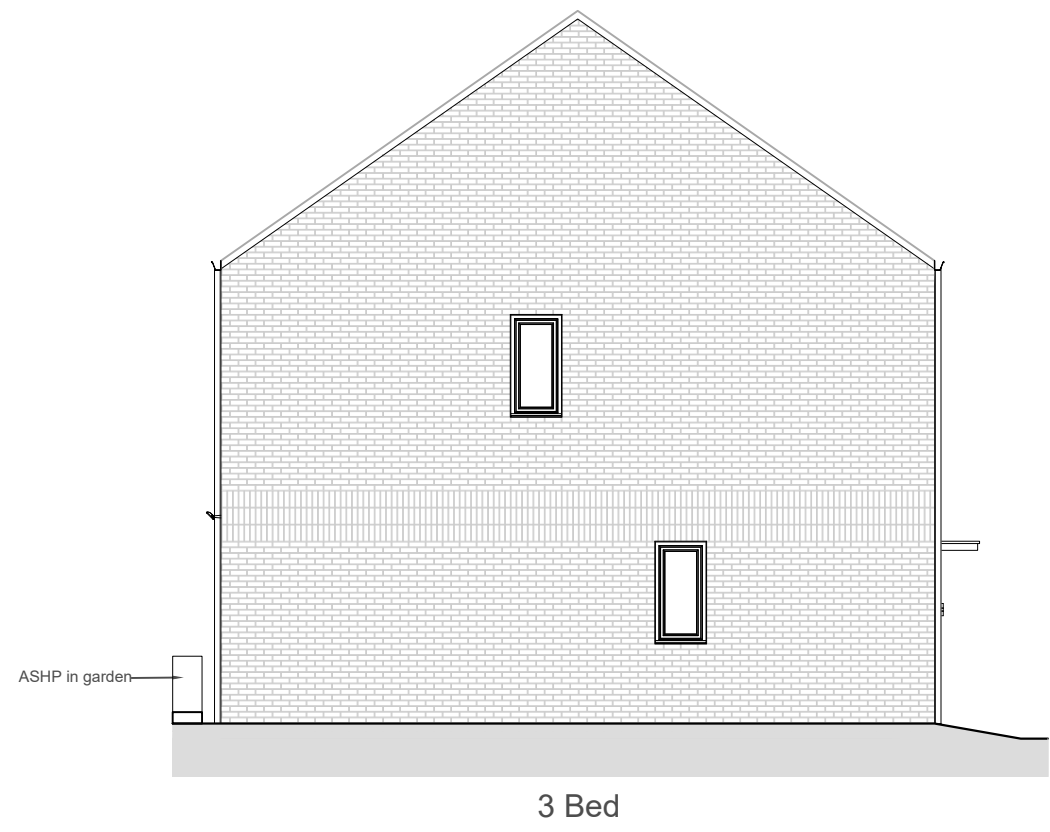
Left Gable Elevation 1:100 * Windows applicable to plots 19 & 29
