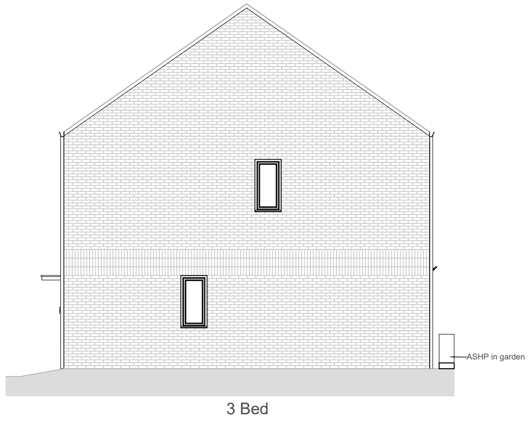
Right Gable Elevation 1:100 * Windows applicable to plots 04 & 27
