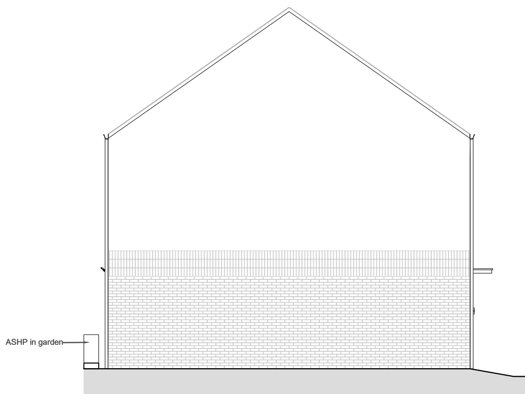
2 Bed Left Gable Elevation 1:100
