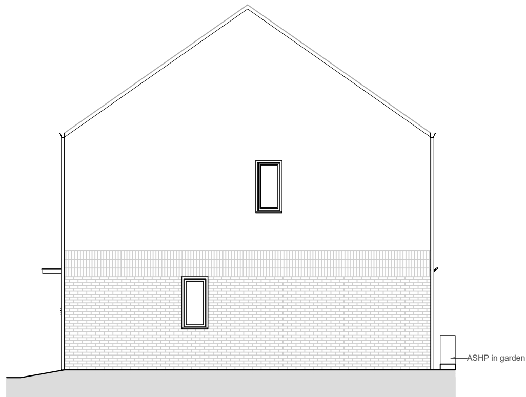
3 Bed Right Gable Elevation 1:100
