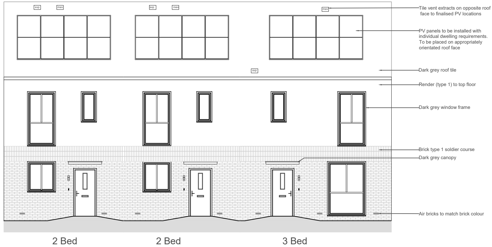
Front Elevation 1:100
