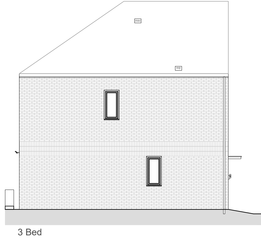
Left Gable Elevation 1:100
