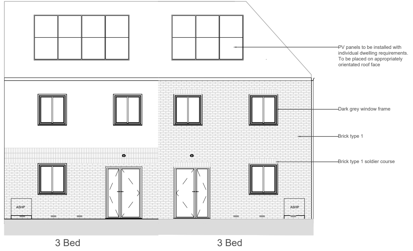
Rear Elevation 1:100
