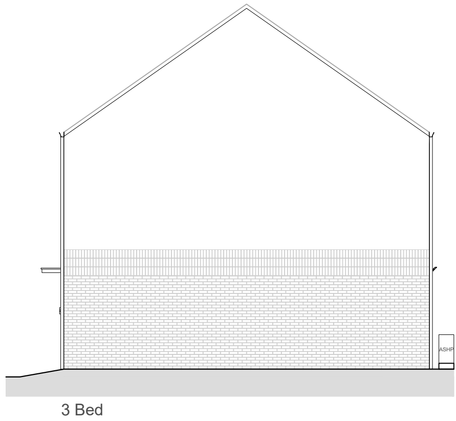
Right Gable Elevation 1:100
