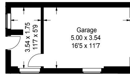
Garage - 24.9 sq m / 268 sq ft
