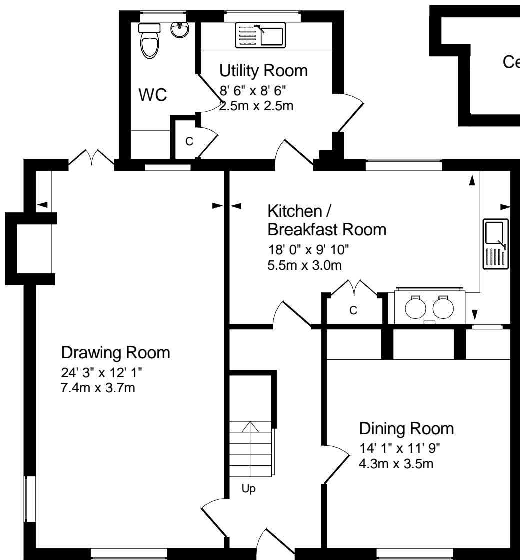
Ground Floor
